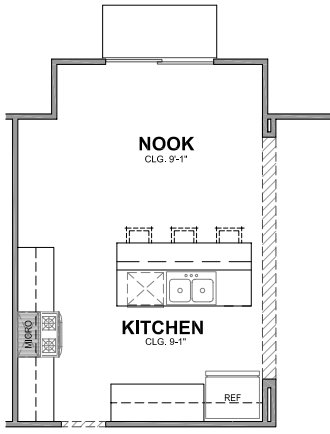
KITCHEN OPTION 1
