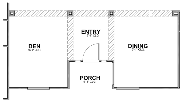
ENTRY COLUMNS OPTION
